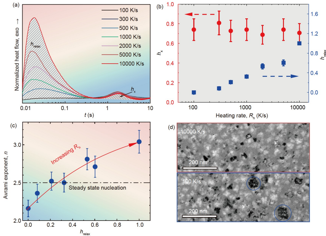
Figure 2 (Color online) (a) Isothermal heat flow curves of as-spun \text{Fe}_{86}\text{B}_{14} at T_a = 773 K with R_h from 100 to 10000 K/s. (b) The normalized crystallization enthalpy ( h_x ) and normalized residual relaxation enthalpy ( h_{\text{relax}} ) estimated from the isothermal curves in (a). (c) The Avrami exponents (for f_t = 20\% -40%) versus h_{\text{relax}} plot estimated from the isothermal curves in (a). (d) Bright field TEM images of \text{Fe}_{86}\text{B}_{14} crystallized isothermally at T_a = 773 K with R_h = 100 K/s ( n = 2.16 , D = 24.4 nm) and R_h = 10000 K/s ( n = 3.04 , D = 20.7 nm), f_t = 80\% -85%.
